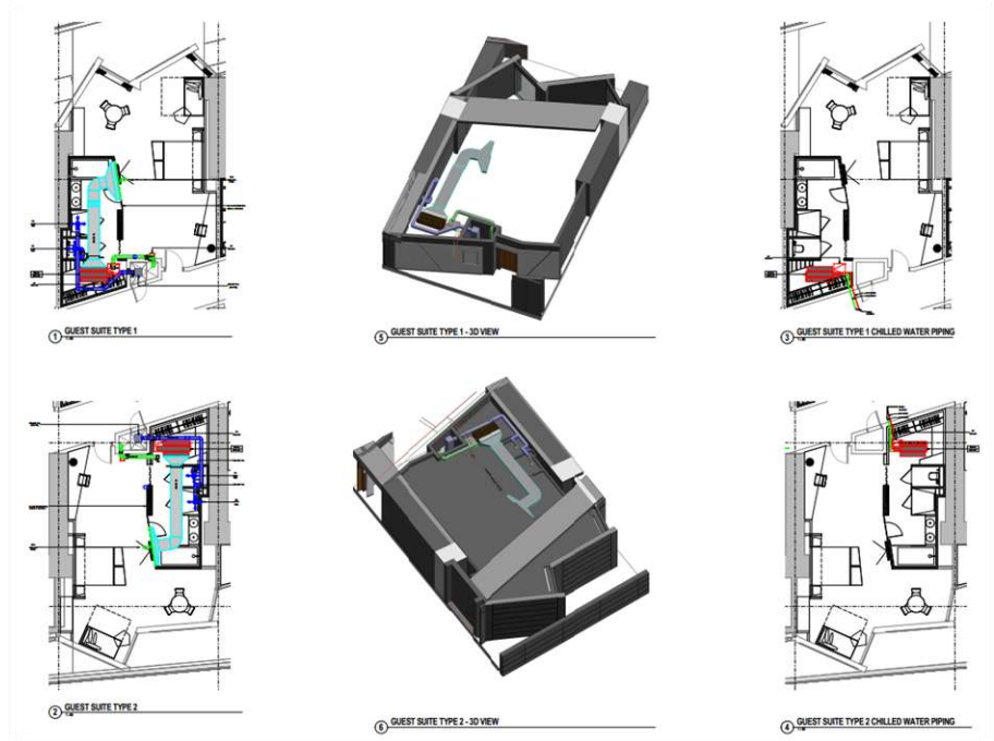
REPRESENTATION OF TYPICAL APPTMENT FOR HOTEL BUILDING
