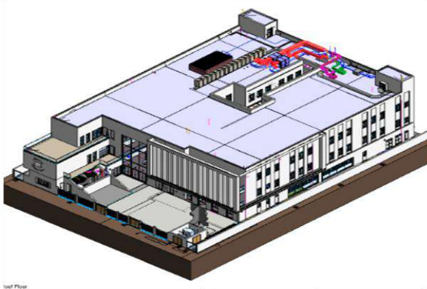
OVERALL BUILDING PRIVATE SCHOOL PROJECT
