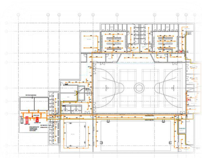
❖ FIRE PROTECTION LAYOUT
