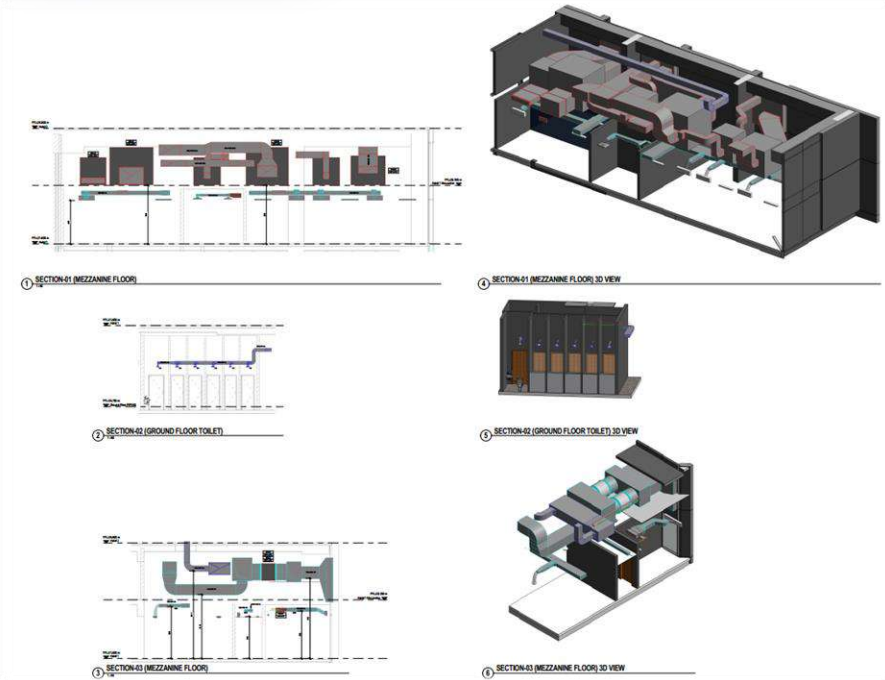
3D VIEWS AND SECTIONS OF CRITICAL AREAS OF HOTEL BUILDING
